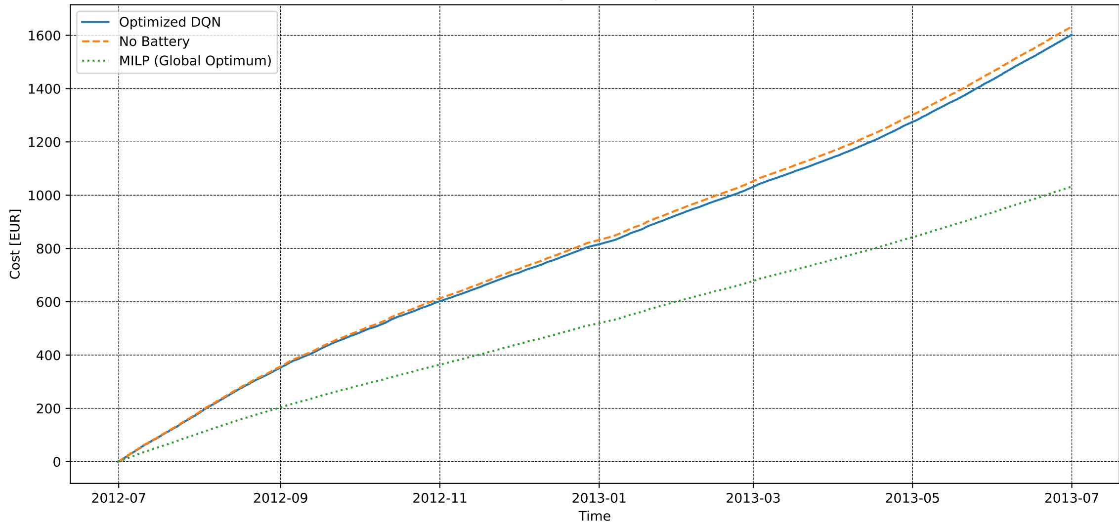
User 249 - Basic Training - Electricity Cost [DQN vs MILP]
